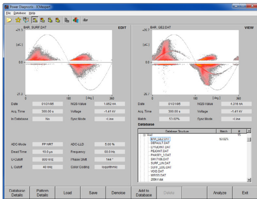
ICMexpert database overview panel
