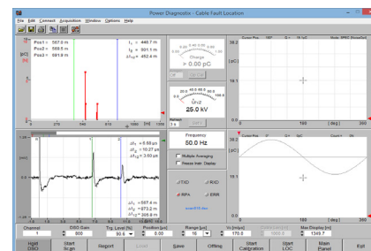
Software panel for cable fault location
